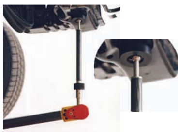
Embout aimanté Magnetic socket for live measuring
